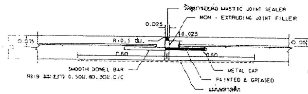
ឧបាយរួមចំ EXPANSION JOINT
