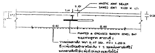
CONTRACTION JOINT
