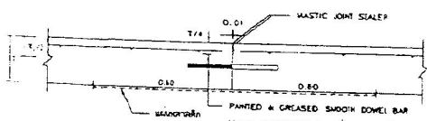
CONSTRUCTION JOINT
