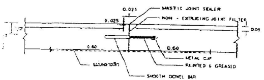
EXPANSION JOINT
